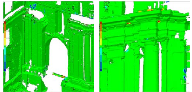
Figure 12. Comparison between the final resulting mesh and the original acquired cloud of points. As side color scale shows, green indicate deviation \leq \pm 0.005\text{ m}
